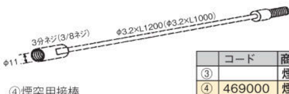
④煙突用接棒
